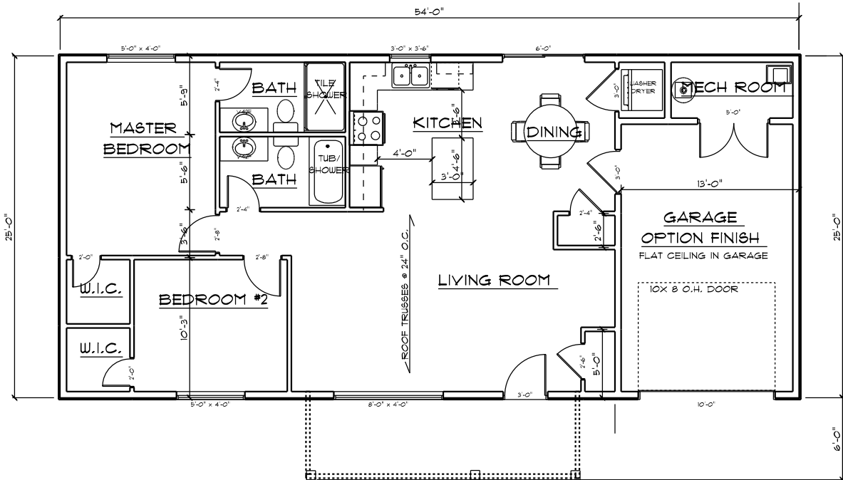
FLOOR PLAN 1013 SQ FT
